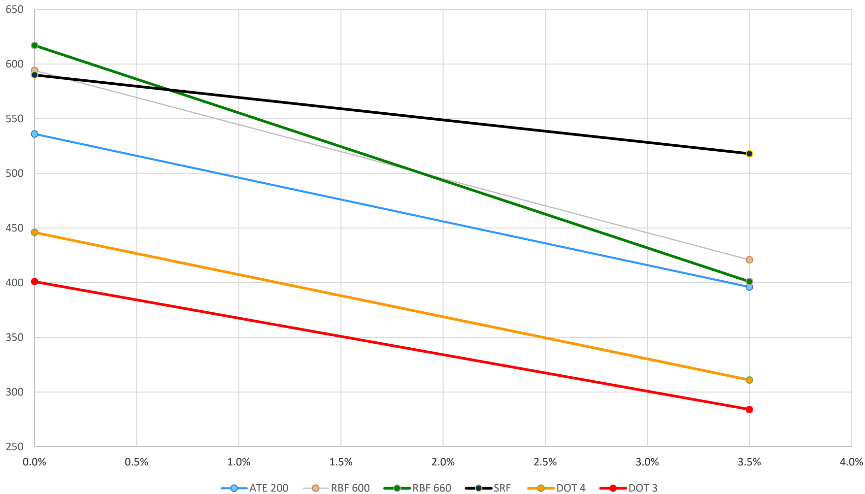
Brake Fluid Boiling Temp vs Moisture Content
